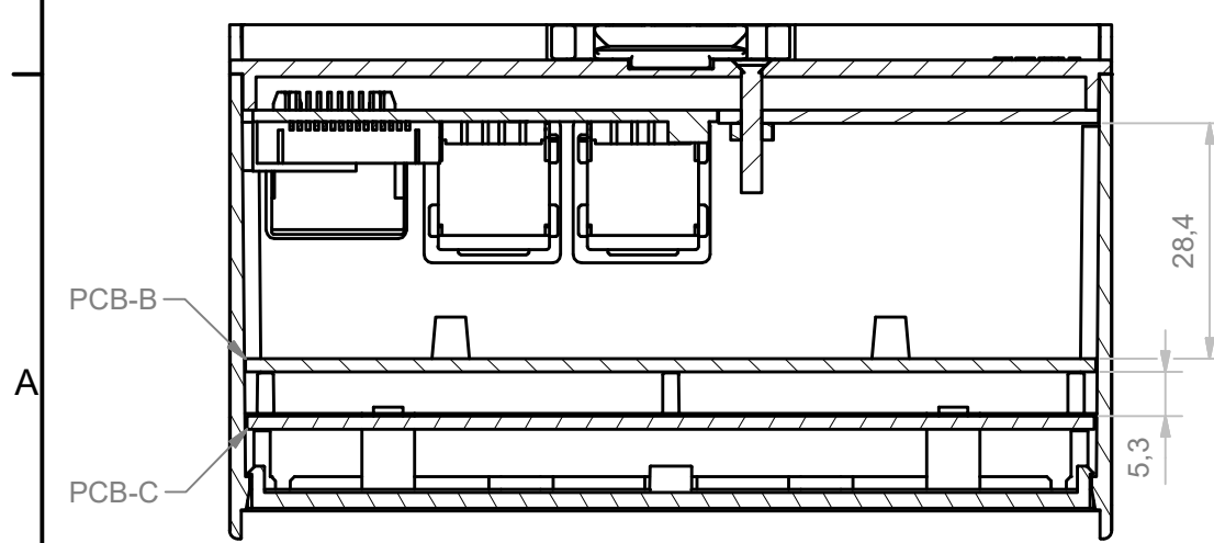
B-B (1:1)
